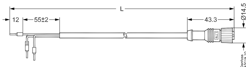
Cable and connector assemblies for ETS with AST-g MK II actuator
